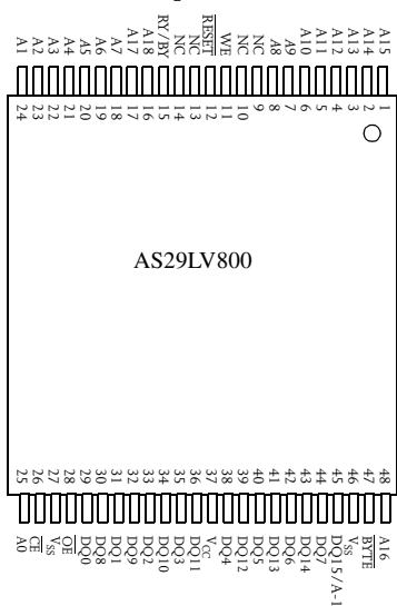
48-pin TSOP
