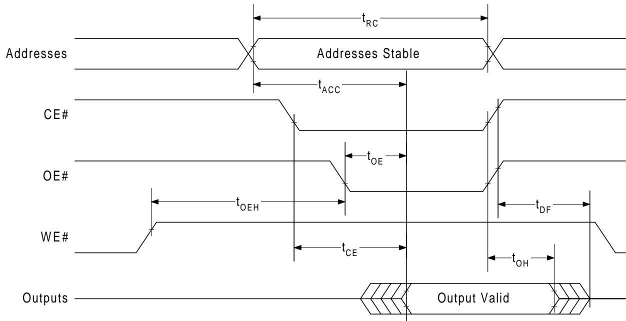
Figure 12. Read Operation Timings
