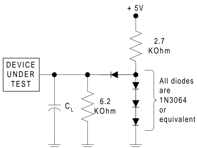
Figure 10. Test Setup
