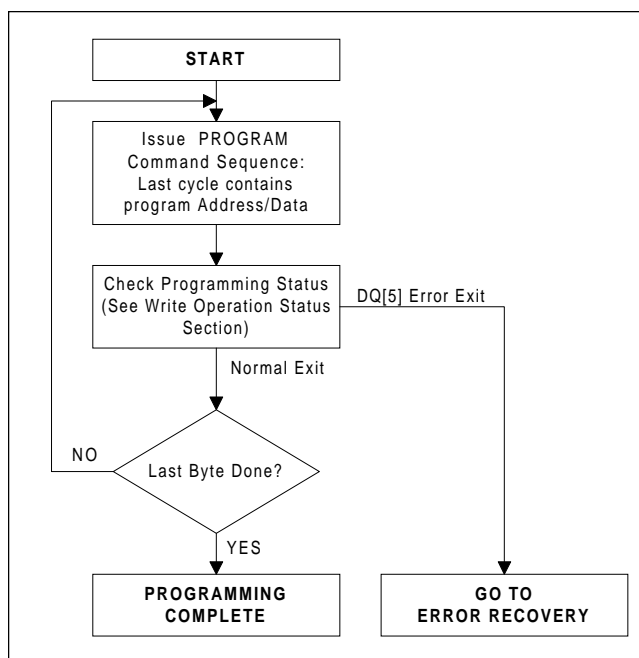
Figure 3. Programming Procedure
